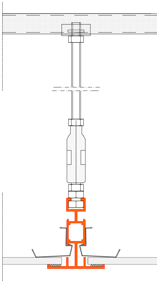
detail A
