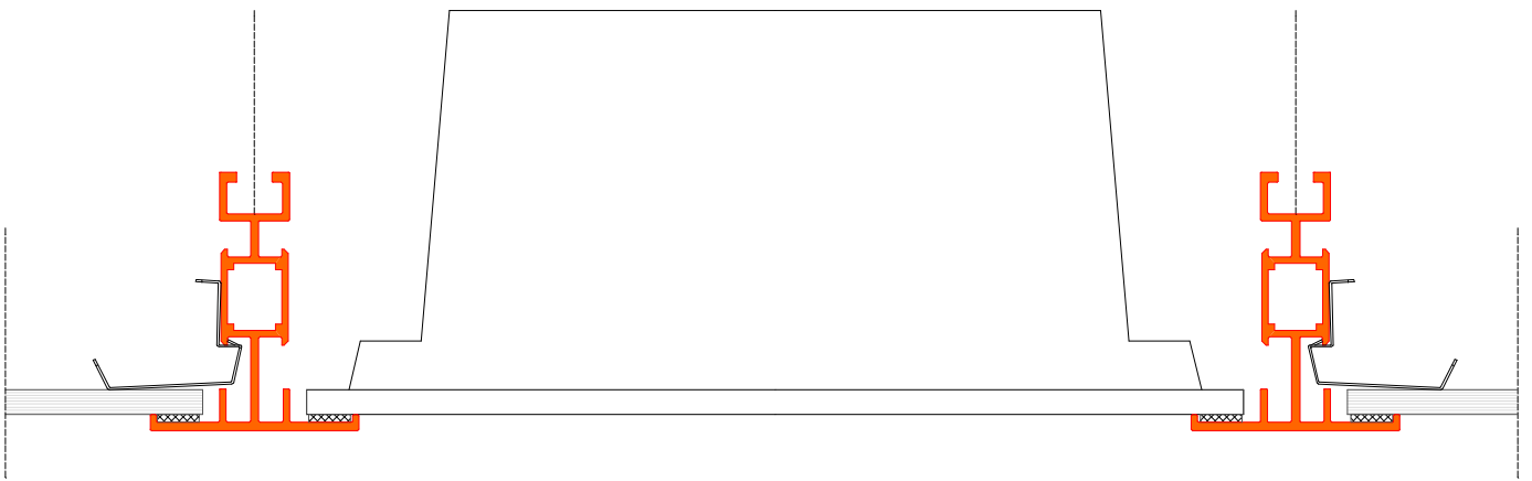
detail A
