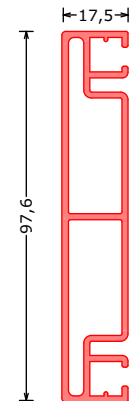
171815*** HPR180ST wandbeëdigingsprofiel recht | cornerprofile 180° square wandstuck 180° rechtwinklich L=6200mm
