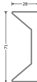
273133000 STA 300 schuifstuk telescoop QW98 | extension telescoop QW98 Schiebeteil telescoop QW98 L=300mm
