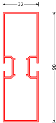
171775*** P1 QW98 P1 profiel QW98 | P1 profile QW98 | P1 Profil QW98 L=6100mm
