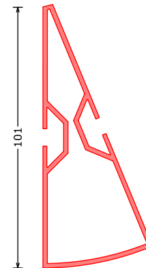
172315*** HP225 QW98 hoekprofiel 22,5° QW98 | cornerprofile 22,5° QW98 Eckprofil 22,5° QW98 L=6100mm
