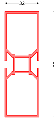
172316*** P2 QW98 P2 profiel QW98 | P2 profile QW98 | P2 Profil QW98 L=6100mm
