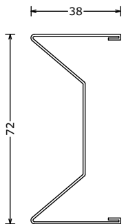
171853*** KOS SPLX omegaprofiel vlak SypLux | coverprofile flas SypLux Omegaprofil flach SypLux L=6100mm
