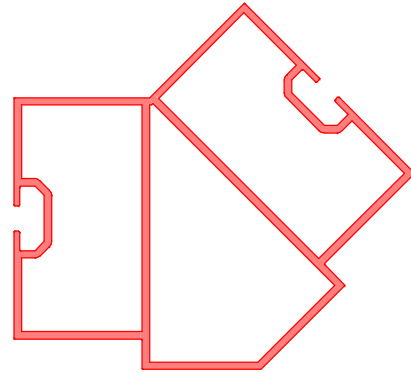
171767*** CP135S CCS-P80 hoekprofiel 135° P80 | cornerprofile 135° P80 Eckprofil 135° P80 L=6100mm
