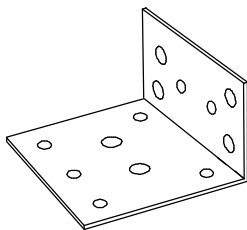
273119000 HA 60*40*60 mm hoekanker 60x40x60mm angle clamp 60x40x60 Eckverbinder 60x40x60
