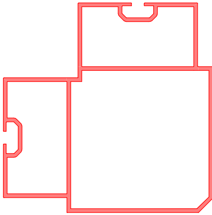
171764*** CP090S CCS-P80 hoekprofiel 90° P80 | cornerprofile 90° P80 Eckprofil 90° P80 L=6100mm
