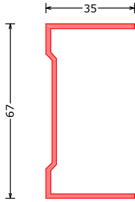
171782*** UP1 64 UP1 profiel vlak QW64 | UP1 profile flat QW64 | UP1 Profil flach QW64 L=6100mm
