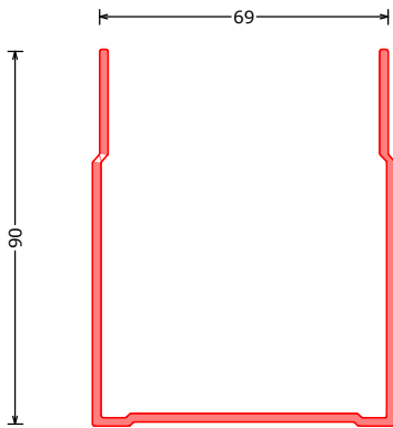
171819*** FP-U090 CLR vloerprofiel 90mm CLR floor profile 90mm CLR Flür Profile 90mm CLR L=6100mm
