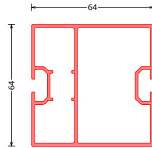
171765*** IP64/64 tussenprofiel 64x64 | intermediate profile 64x64 Zwischenprofil 64x64 L=6100mm
