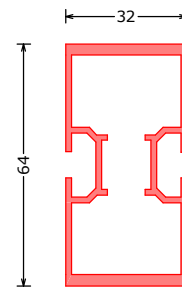
171783*** P1 64 P1 profiel QW64 | P1 profile QW64 | P1 Profil QW64 L=6450mm
