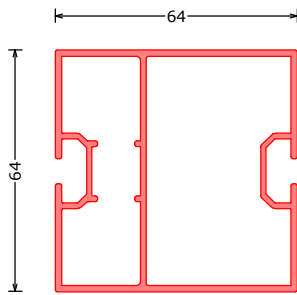
171765*** IP64/64 tussenprofiel 64x64 | intermediate profile 64x64 Zwischenprofil 64x64 L=6100mm
