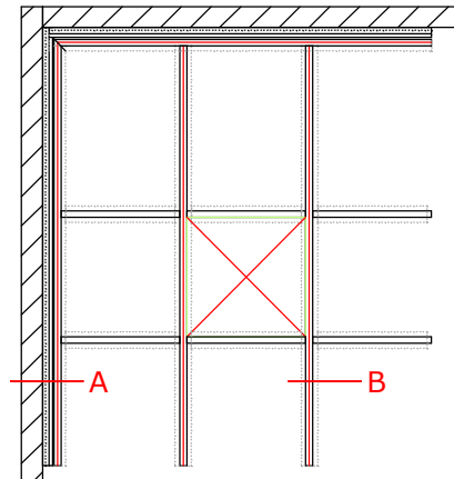
CCS C80-CPO cleanroom system
