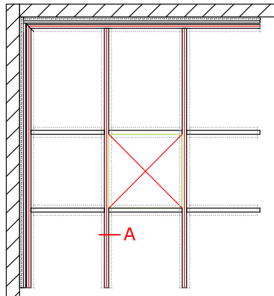
CCS C80-CPC cleanroom systeem
