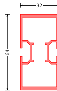
171800*** P1 37 P1 profil QW37 | P1 profile QW37 | P1 Profil QW37 L=6450mm
