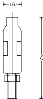
2733356000 pendelophanger M8 Swevel hanger M8 Pendelaüfhänger M8
