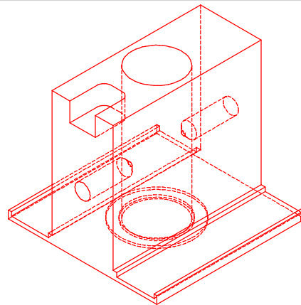
273043*** S-bloc CPO/ CPC CCS-C80 electra doorvoerblok voor CPC/ CPO PS78DFC sprinkler transit profile for CPC/ CPO PS78DFC sprinkler Transit Profil für CPC/ CPO PS78DFC L=78mm
