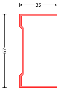
171799*** UP1 37 UP1 profil vlak QW37 | UP1 profile flat QW37 | UP1 Profil flach QW37 L=6100mm
