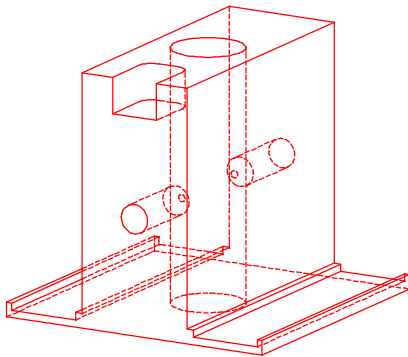
273043*** E-bloc CPO/ CPC CCS-C80 electra doorvoerblok voor CPC/ CPO PS78DFC electra transit profile for CPC/ CPO PS78DFC electra Transit Profil für CPC/ CPO PS78DFC L=78mm
