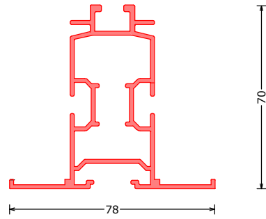
171759*** CPO CCS-C80 plafondprofiel open 78mm PS78DFC L=6000mm
