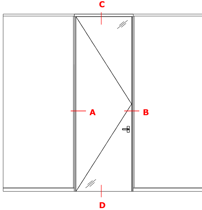
TecnoLine : modul DAW-HG
