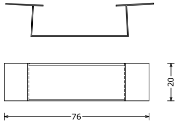
273934000 FS TL98 fixeerbeugel TecnoLine fixationclip TecnoLine Fixierbügel TecnoLine
