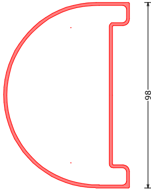
171772*** HP180ST wandbeëdigingsprofiel rond | cornerprofile 180° wandbeëdigings profiel 180° L=6200mm
