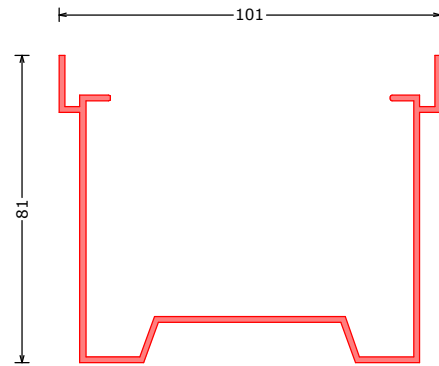
171786*** VP vloerprofiel | floor track | Bodenprofil L=6100mm
