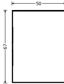
273695000 CST50 TL98 2575 CST50 staander 2575 TecnoLine CST50 steel stud 2575 TecnoLine CST50 Ständer 2575 TecnoLine L=2575mm
