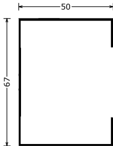
273691000 CST50 TL98 2775 CST50 staander 2775 TecnoLine CST50 steel stud 2775 TecnoLine CST50 Ständer 2775 TecnoLine L=2775mm
