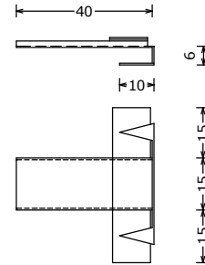
273935000 SC TL98 slagclip TecnoLine steel panel clamp TecnoLine Schlagclip TecnoLine
