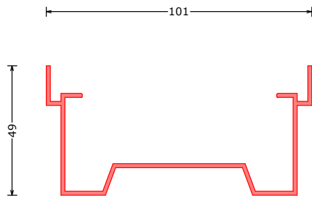
171829*** VP49 vloerprofiel 49mm | floor track 49mm | Bodenprofil 49mm L=6100mm
