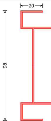
171788*** WA wandaansluiting | wall connection profile | Wandanschlußprofil L=6100mm
