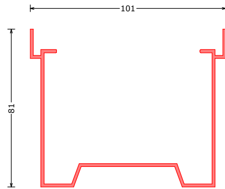
171786*** VP vloerprofiel | floor track | Bodenprofil L=6100mm
