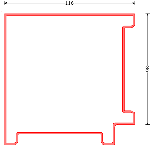
171817*** HPR90ST hoekprofiel recht 90° | corner profile 90° square | Eckprofile 90° rechtwinklich L=6200mm
