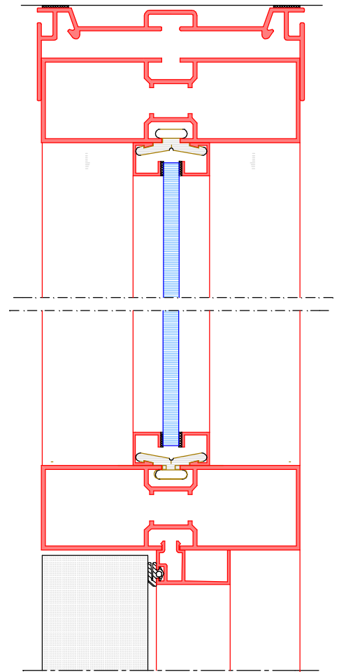
detail C
