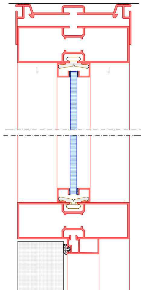
detail C
