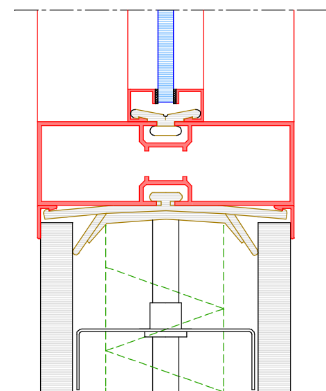
detail C
