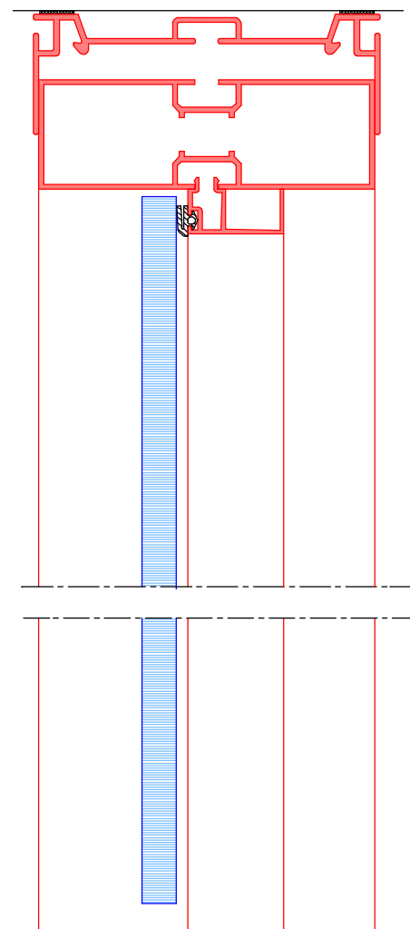
detail C
