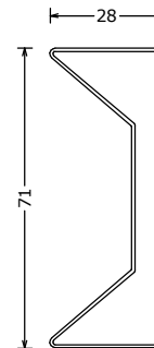
172035*** T1-35 omegaprofiel T1 vlak | cover profile T1 flat | Abdekprofil 35mm flach L=6100mm
