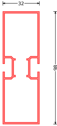
171775*** P1 QW98 P1 profiel QW98 | P1 profile QW98 | P1 Profil QW98 L=6100mm
