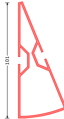
172315*** H225 QW98 hoekprofiel 22,5° QW98 | cornerprofile 22,5° QW98 Eckprofil 22,5° QW98 L=6100mm
