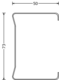
243233000 C73 3000 ST98-SMS C73 3000 ST98-SMS | C73 3000 ST98-SMS | C73 3000 ST98-SMS L=3000mm
