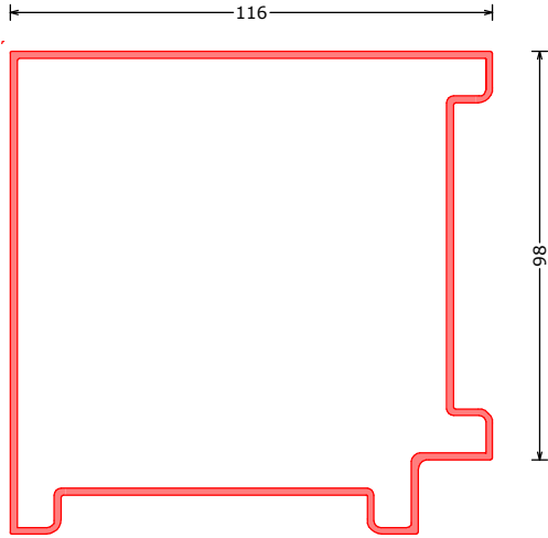
171817*** HPR90ST hoekprofiel recht 90° | corner profile 90° square | Eckprofile 90° rechtwinklich L=6200mm
